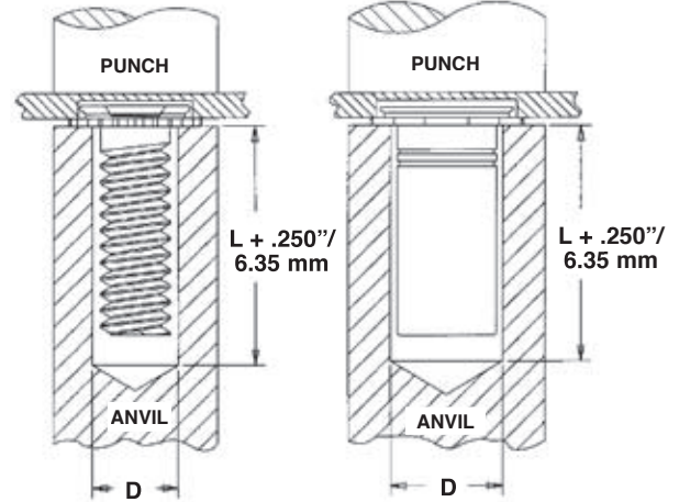
Types CFHA, CFHC, CHC, CHA Concealed-head studs
